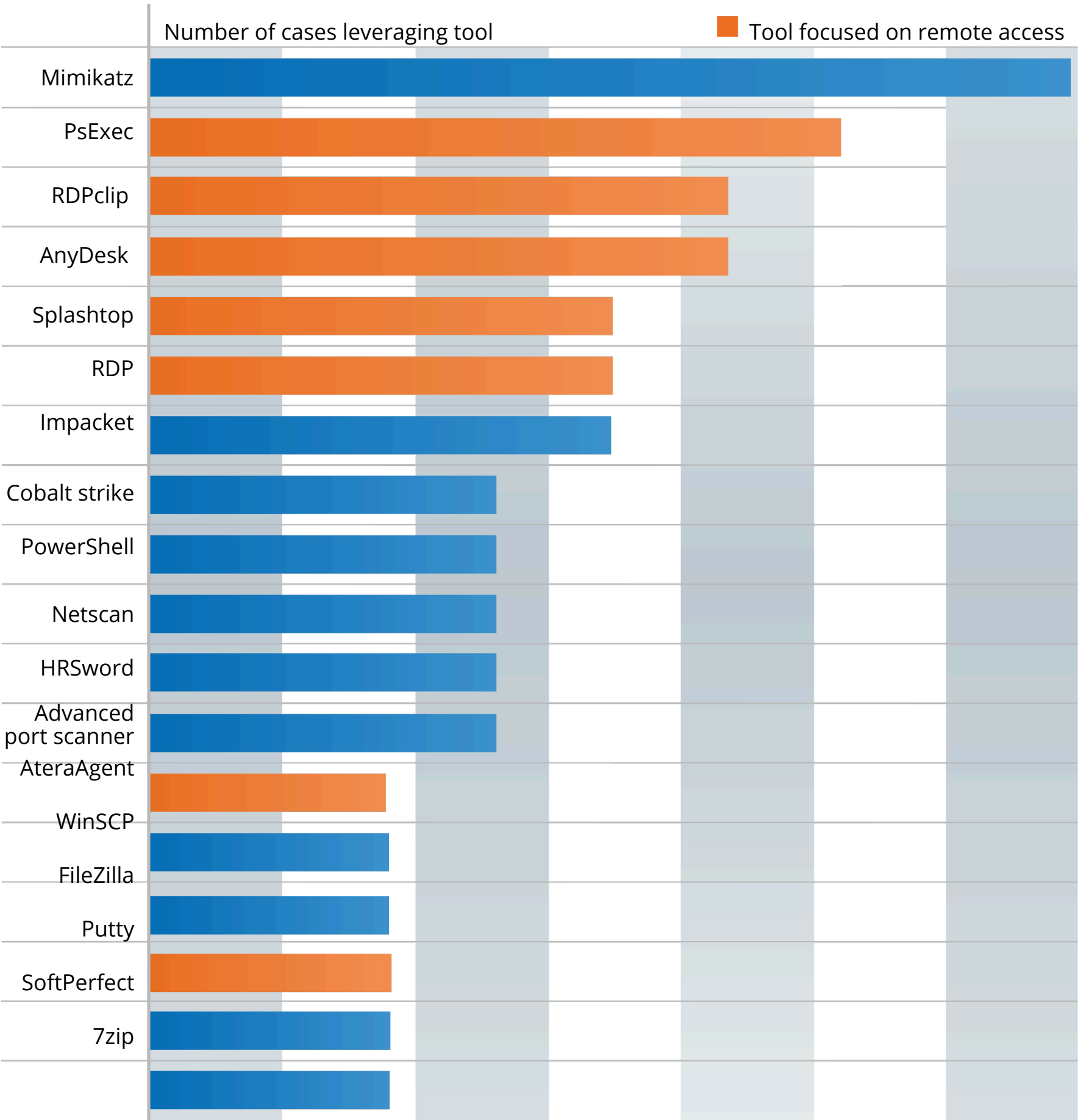
Figure 17 Top tools seen in Talos IR ransomware engagements
