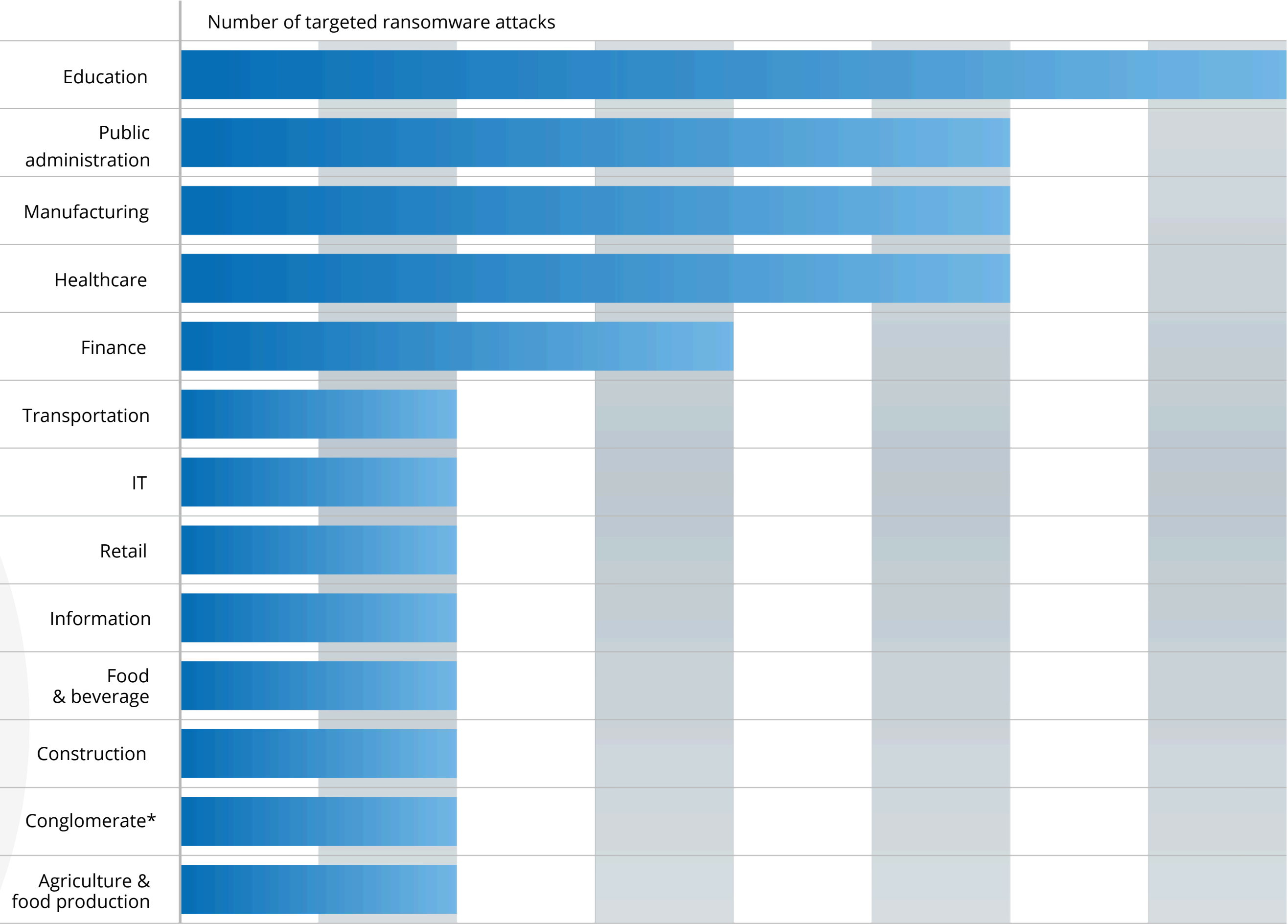
Figure 12 Targeted sectors
