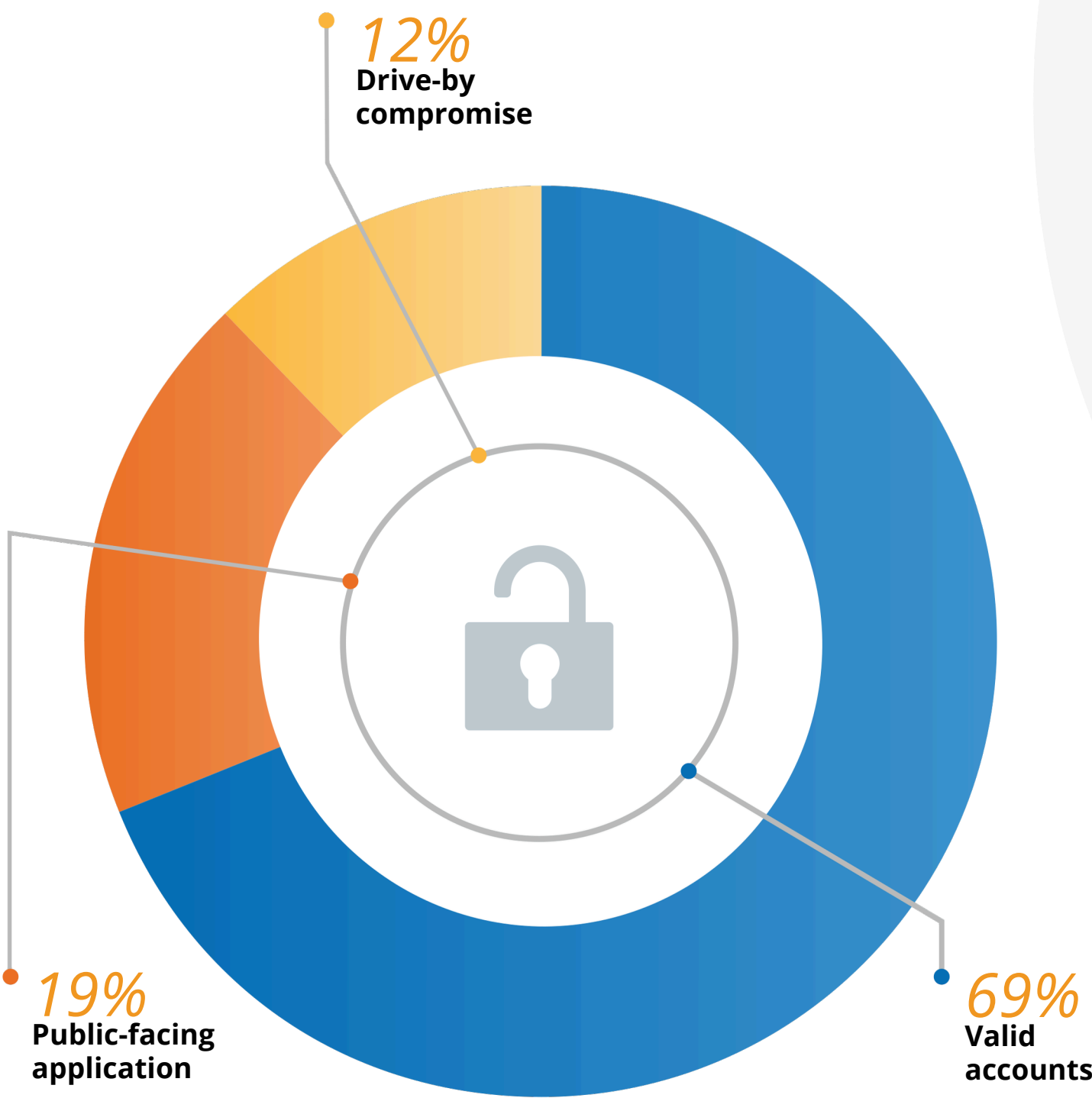
Figure 16 Initial access
