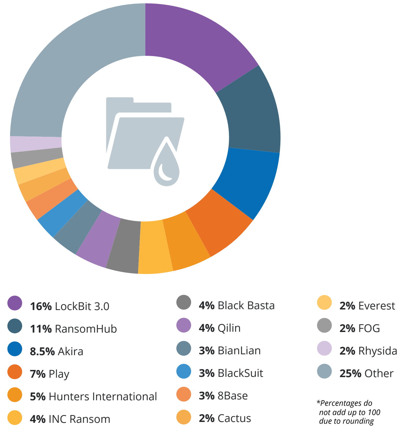
Figure 18 2024 volume of posts made to data leak sites by ransomware groups
