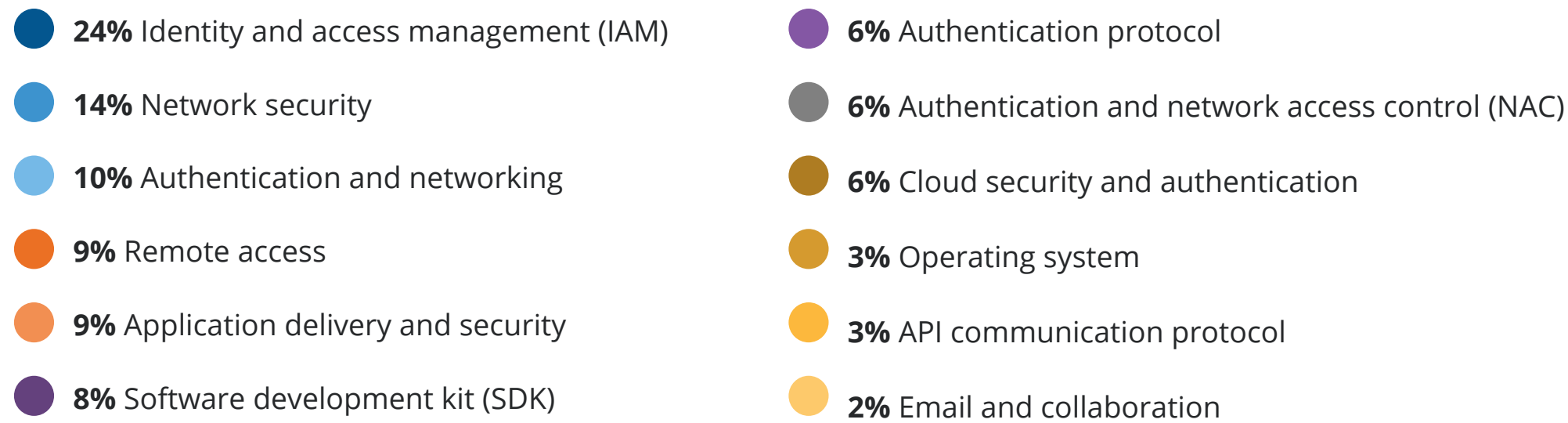
Figure 21 Types of applications targeted in MFA attacks
