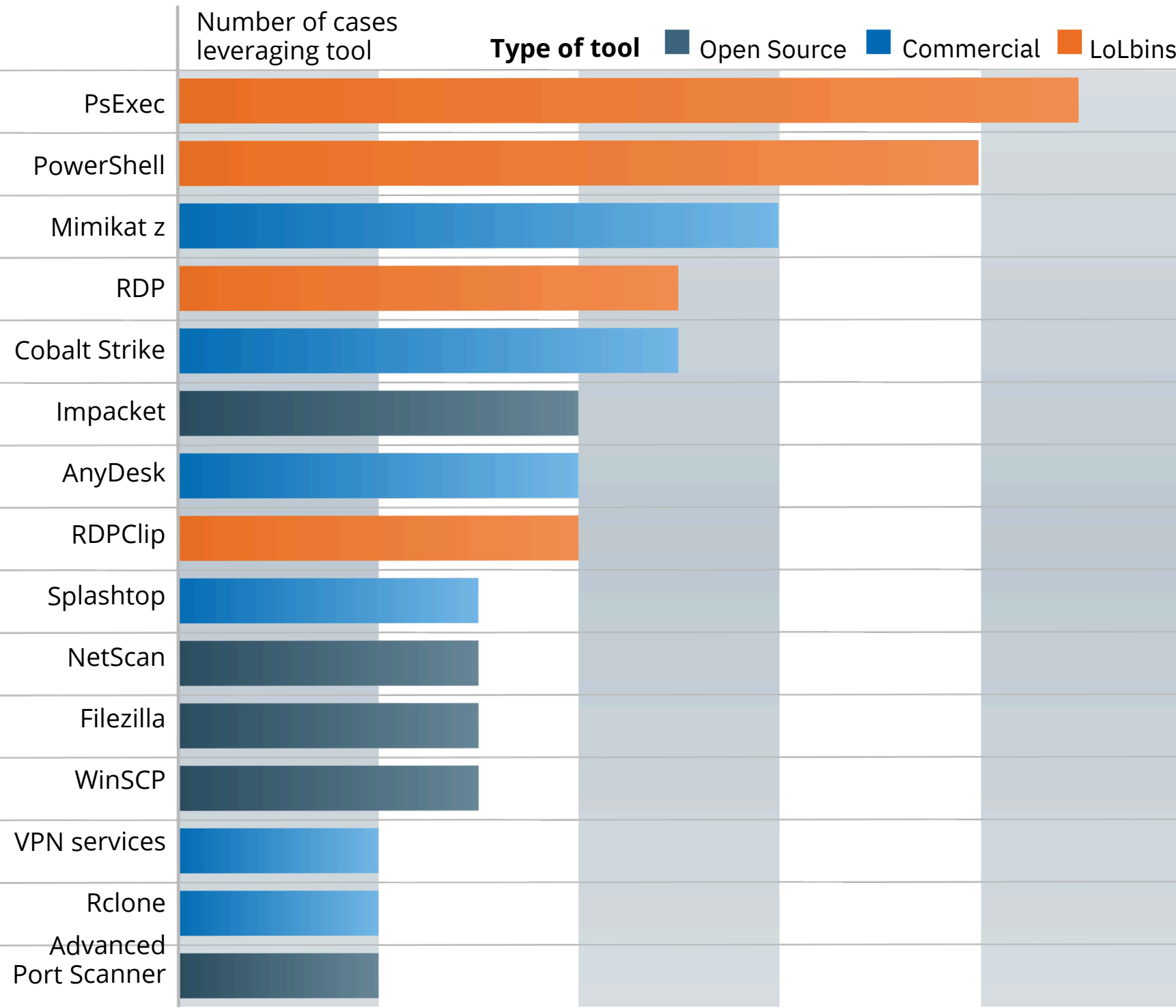
Figure 11 LoLBins used across the attack chain in Talos IR incidents
