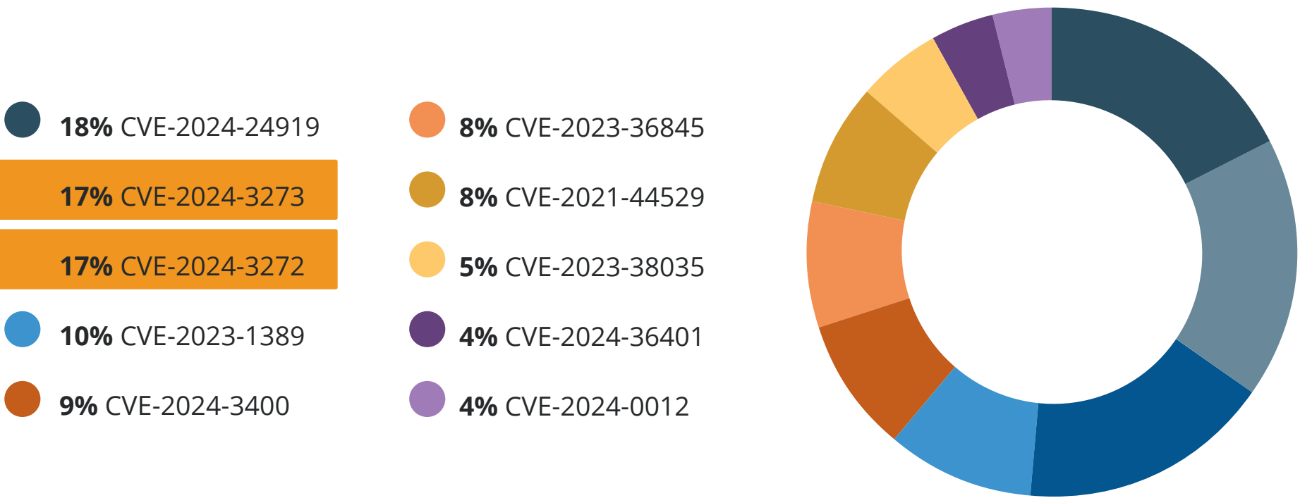
Figure 3 Top-targeted network device CVEs
